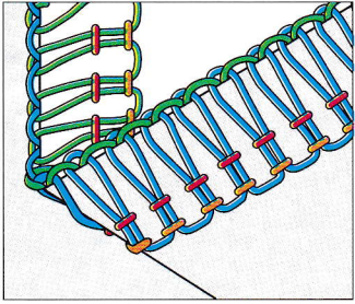
Four thread overlock stitch
