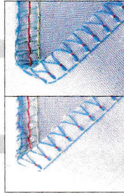
Upperlooper thread is tight.
