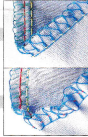
Left needle thread is tight.
